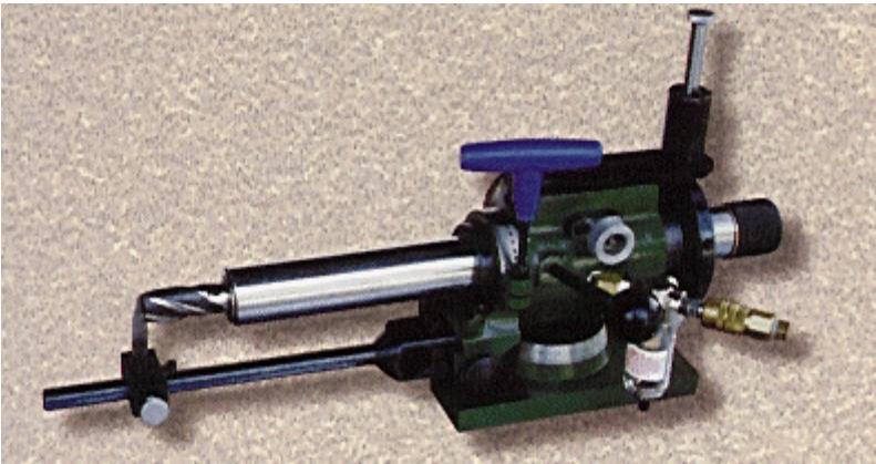
Air Bearing Fixture on Universal Base shown
